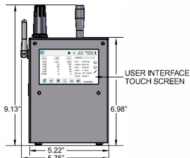
Configurable Environmental Sensor Display
